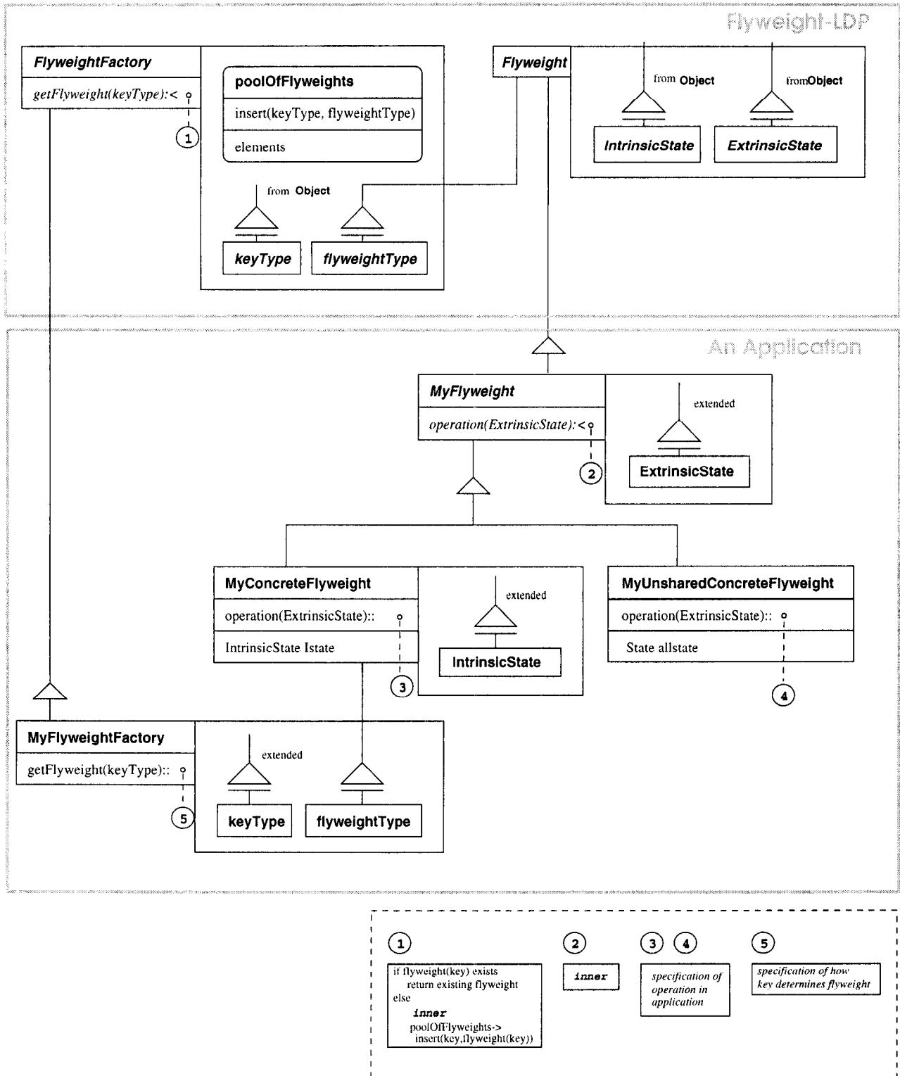
Figure 8: Flyweight-LDP
