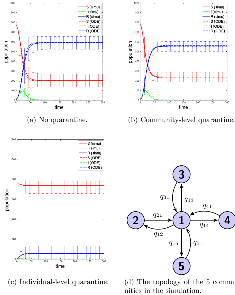
Fig. 4. The simulation result and the community topology of the flu spread model
