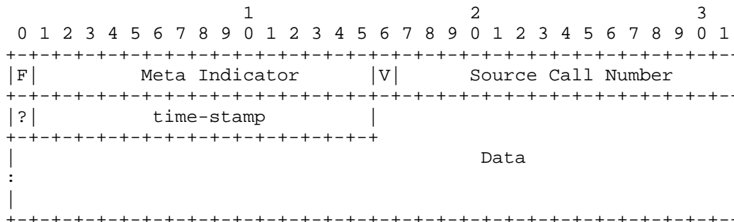
Figure 7: Meta Video Frame Binary Format
