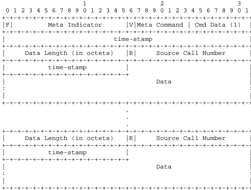
Figure 9: Meta Trunk Frame Binary Format (trunk time-stamps 1)
