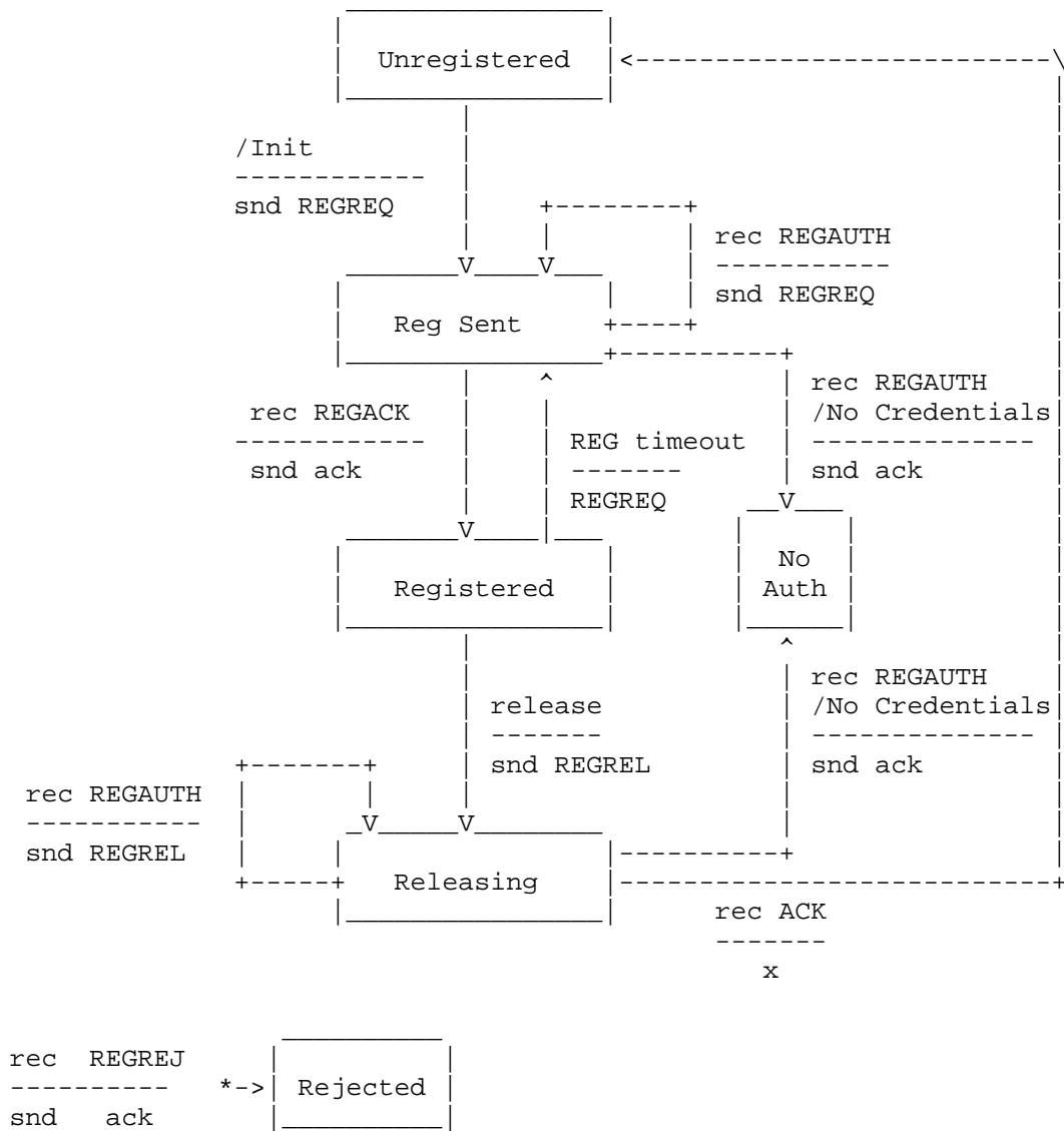
Figure 1: Registrant State Diagram
