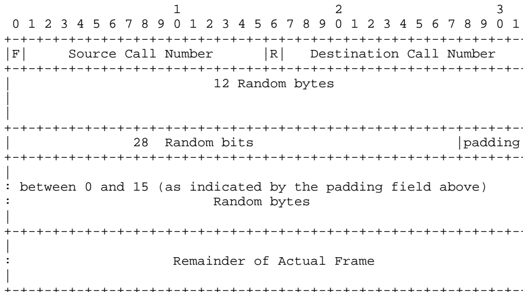
Figure 10: Full Frame before encryption
