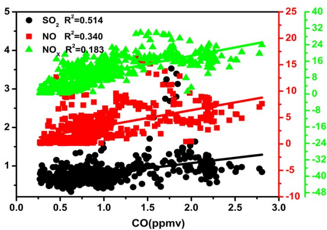
Fig. S2 Correlations of CO with SO 2 , NO and NO x in urban site (top) and suburban
