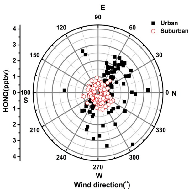
Fig.S1 The distribution of HONO with the wind directions
