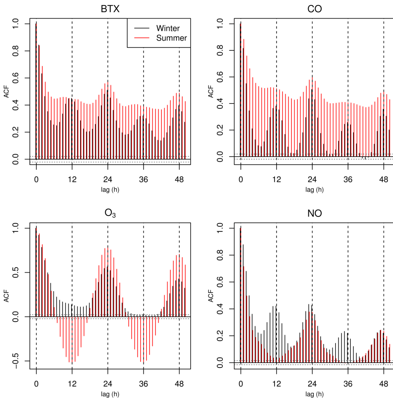
Figure S1. Autocorrelation function for mean hourly concentration data
