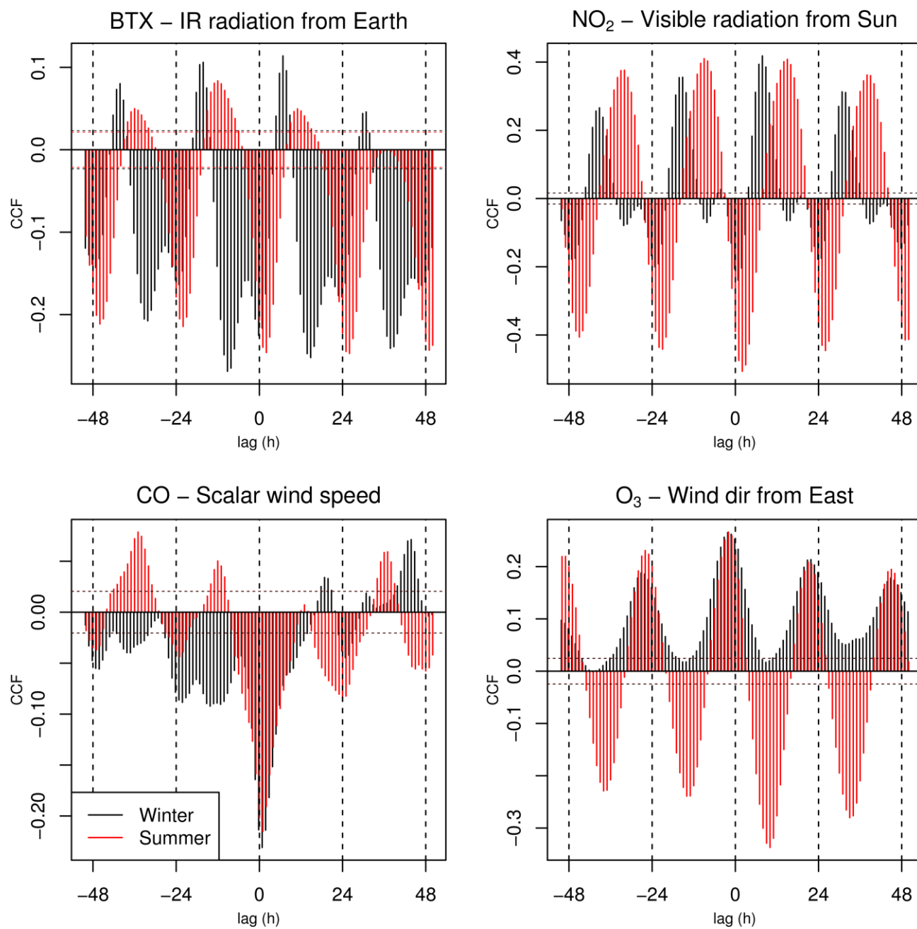
Figure S2. Cross correlation function for hourly concentration data and meteorological variables
