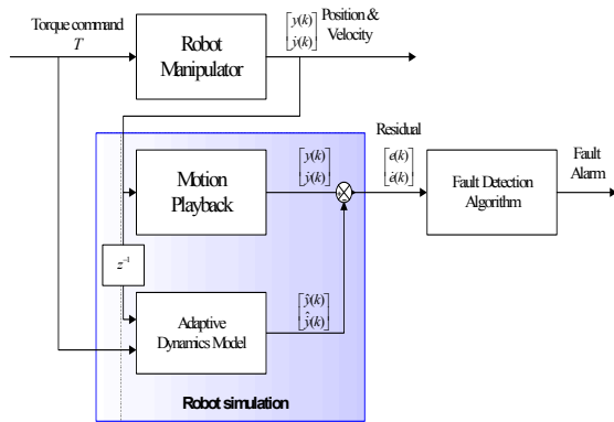
Figure 4: Monitoring and fault detection scheme for the actuators and mechanics of a robot manipulator.
