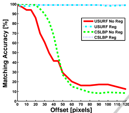
Figure 7: Matching performance with and without image alignment.
