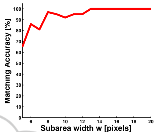
Figure 8: The effect of subarea width on matching accuracy for CS-LBP method (100 board sample size, total of 15 subwindows).
