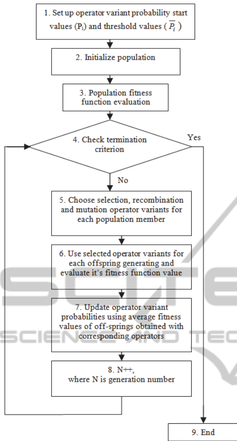
Figure 1: Main part of SelfCEA block diagram.
