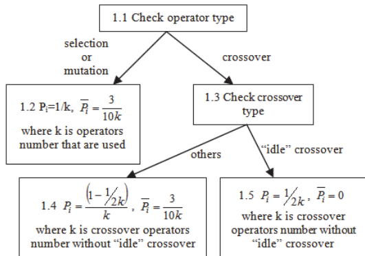
Figure 2: Flowchart illustrating step 1 in SelfCEA block diagram.
