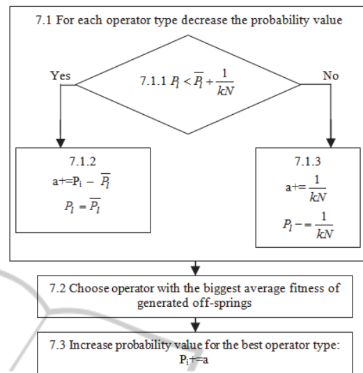
Figure 3: Flowchart illustrating step 7 in SelfCEA block diagram.
