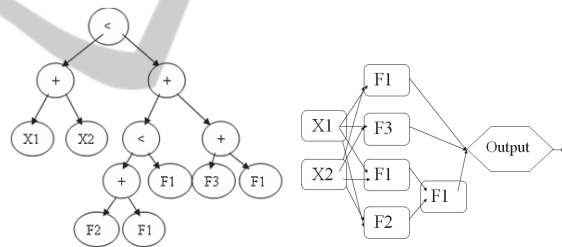
Figure 4: Tree and corresponding neural network example.
