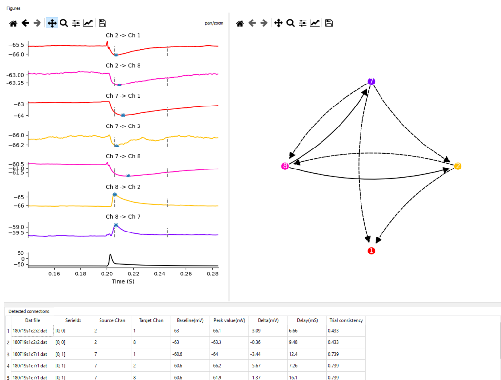
Figure 3: PatchView synaptic connection analysis GUI. Middle left: data series browser. It lists series recorded in a set of synaptic connection experiments from a group of neurons simultaneously recorded in the same slice. Top right: the left plot shows averaged traces of stimuli invoked responses. titles show the channel names of pre and post neurons. The right plot is a graph representation of detected connections. Bottom right panel: quantification of detected connections: including peak voltage, peak height, peak delay, trial consistency.
