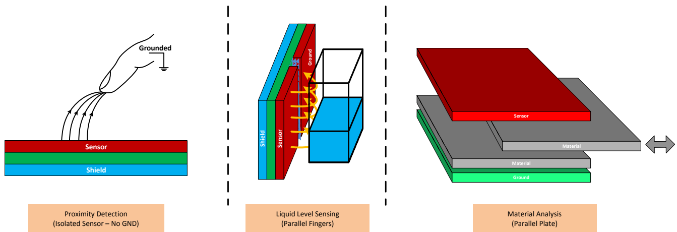
Figure 2-1. Basic Implements for Capacitive Sensing
