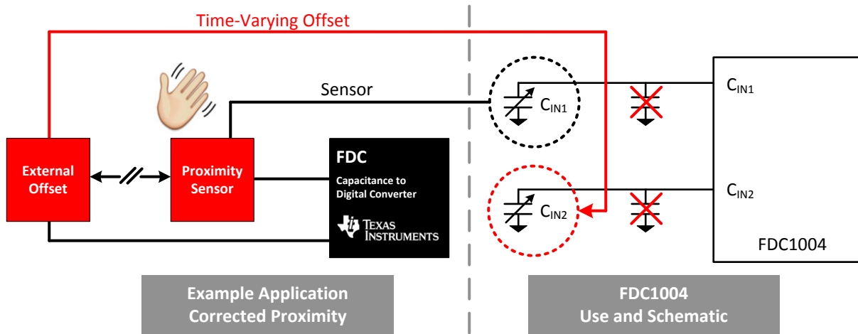
Figure 5-4. Time-Varying Offset Measurements Example
