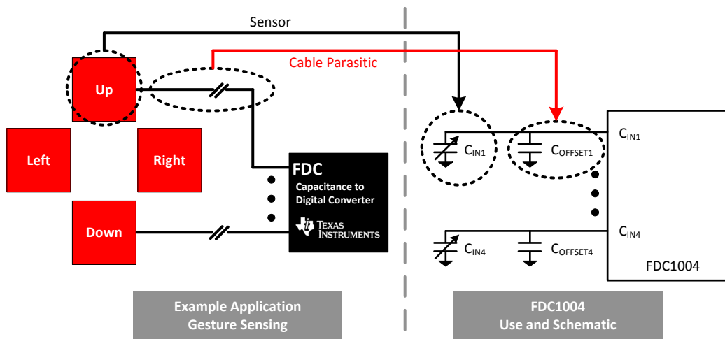
Figure 5-1. Independent Channel use Case for Gesture Sensing Application
