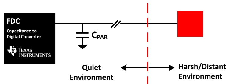
Figure 5-3. Remote Sensing Example
