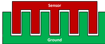
Figure 6-4. Comb Sensor Design
