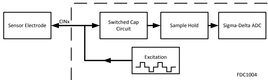
Figure 4-1. FDC1004 Capacitive Sensing Theory of Operation
