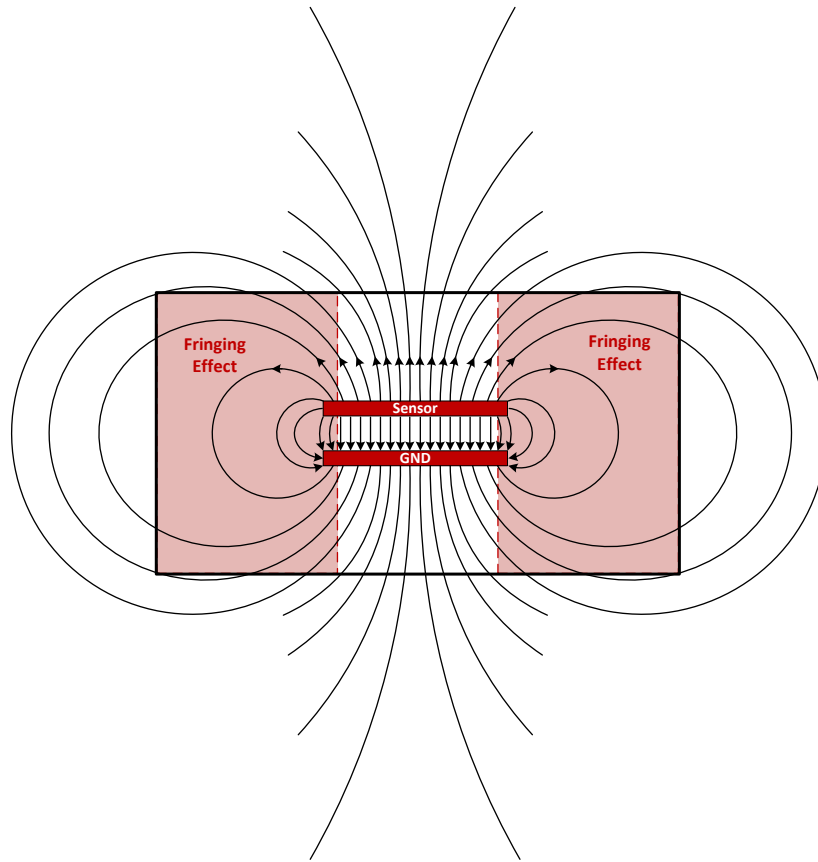
Figure 1-2. Electric Fields of a Parallel Plate Capacitor
