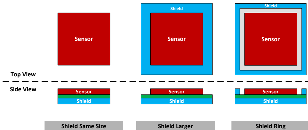
Figure 7-1. Shield Configurations
