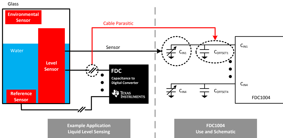
Figure 5-2. Differential or Ratiometric Measurements Example, Liquid Level
