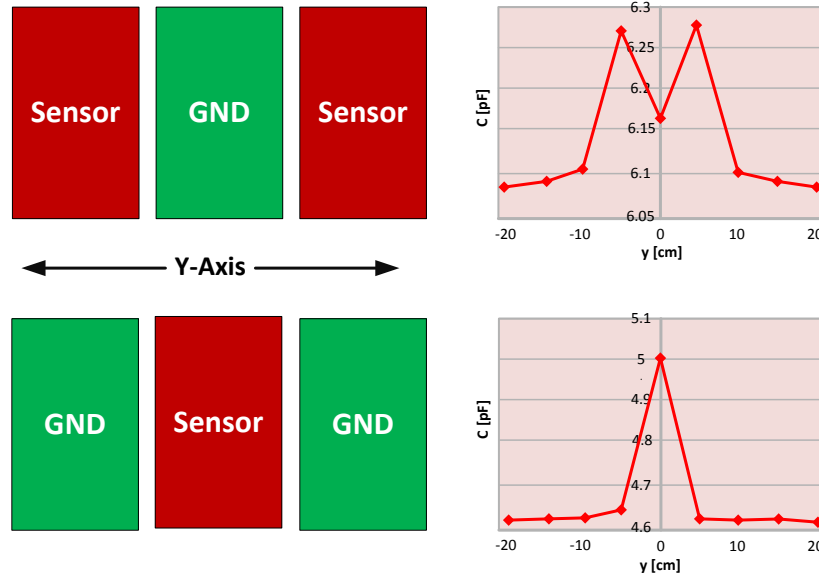
Figure 6-3. Central Ground, Central Sensor Symmetry
