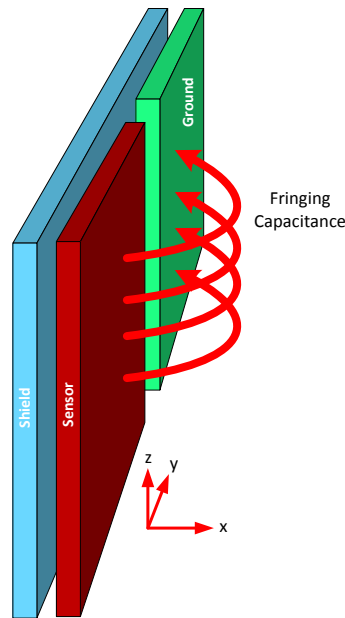
Figure 6-2. Parallel Fingers (GND-Sensor) Topology
