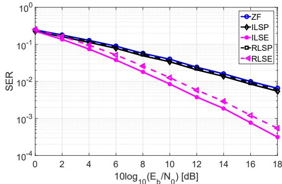
Fig. 3: SER for a 2 \times 2 OFDM system, \Delta F = 3 , N = 128 , K = 8 .
