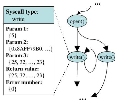
Figure 4: An example system call graph.
