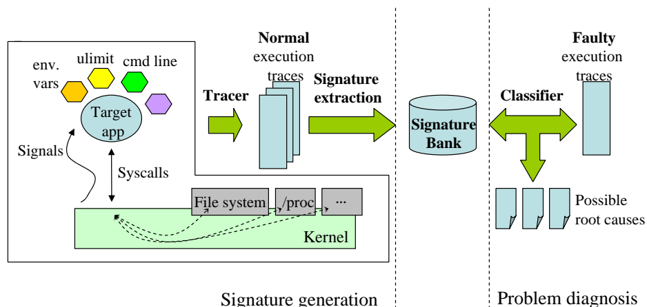
Figure 7: System architecture.
