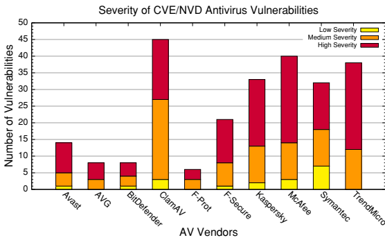
Figure 2: Number of vulnerabilities reported in the National Vulnerability Database (NVD) for ten antivirus vendors between 2005 and November 2007
