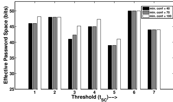
Figure 11: Password Space reduction
