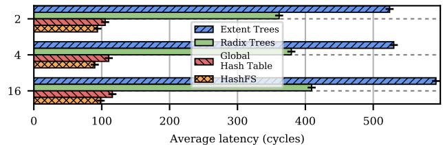
Figure 10: Average file mapping latency, varying # of threads.
