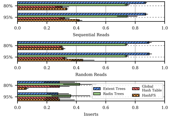
Figure 9: Space utilization test, measuring the proportion of the IO path spent in file mapping versus the overall utilization of the file system (in percent).
