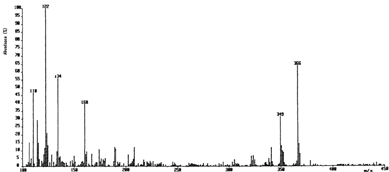
Figure 6. Positive ion mass spectrum of amoxicillin trihydrate
