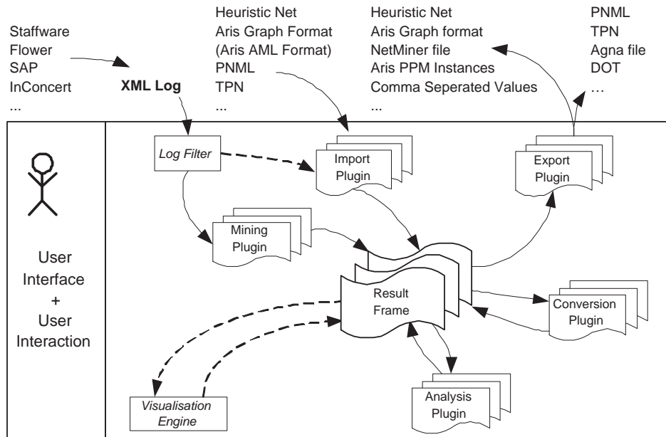
Fig. 2. Overview of the ProM framework
