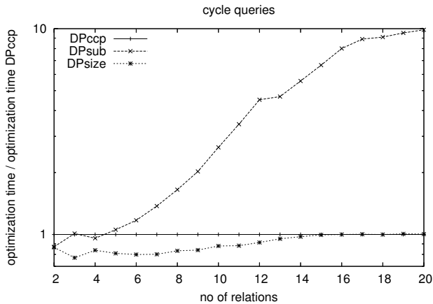
Figure 9: Relative performance for cycle queries
