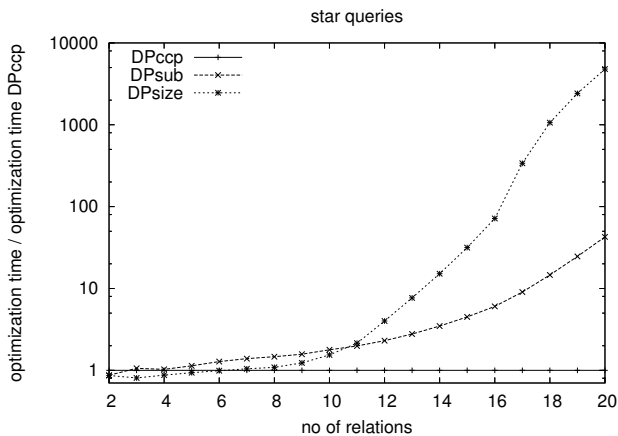
Figure 10: Relative performance for star queries
