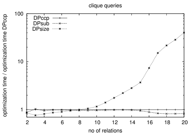
Figure 11: Relative performance for clique queries
