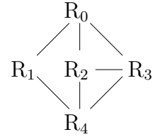
Figure 6: Sample graph to illustrate EnumerateCsgRec
