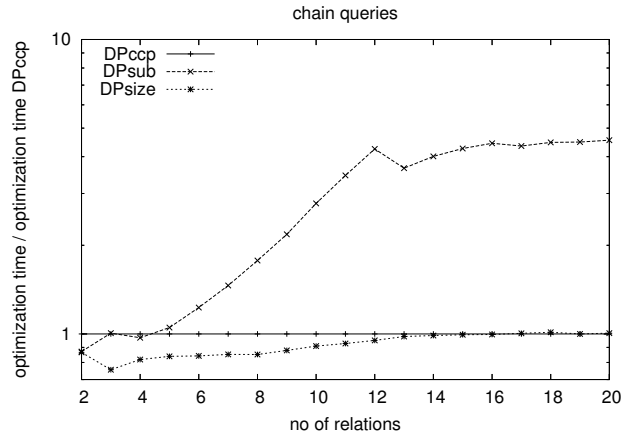
Figure 8: Relative performance for chain queries
