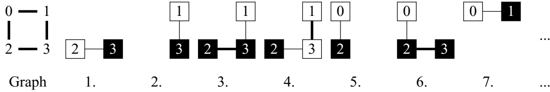
Figure 5: Enumeration Example for DPccp
