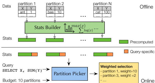
Figure 1: Our system PS 3 makes novel use of summary statistics to perform importance and similarity-aware sampling of partitions.
