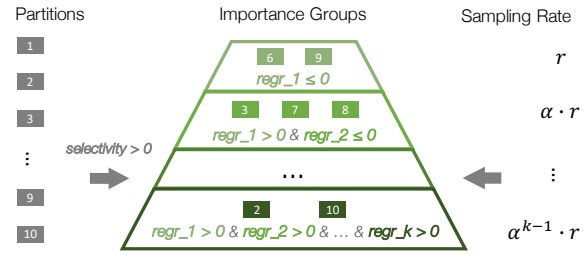
Figure 2: The trained regressors are used to classify input partitions into groups of different importance. The sampling rate decreases by a factor of \alpha > 1 from the i^{\text{th}} important to the (i + 1)^{\text{th}} important group.
