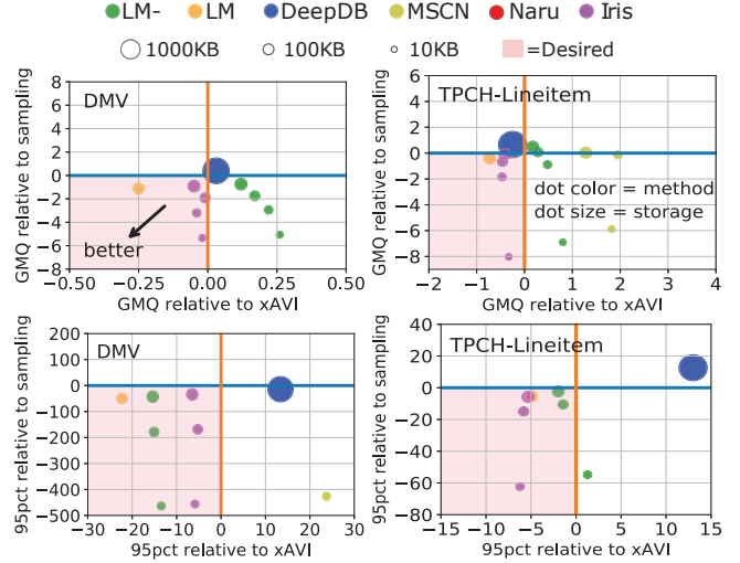
Figure 9: The relative change in accuracy (GMQ and 95 percentile) for different CE techniques over two simple production baselines (Sampling and xAVI); we show summary sizes that are \frac{1}{4} \times - 2 \times of the storage used in production systems.
