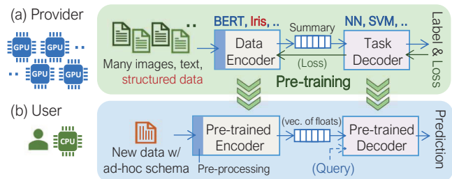
Figure 2: Building and applying pre-trained models. Iris provides off-the-shelf models for structured datasets.
