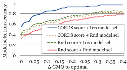
Figure 12: On Lineitem with 1× storage, for different model selection schemes, we show their accuracy to pick summaries that are within \Delta GMQ ( x -axis) to optimal.
