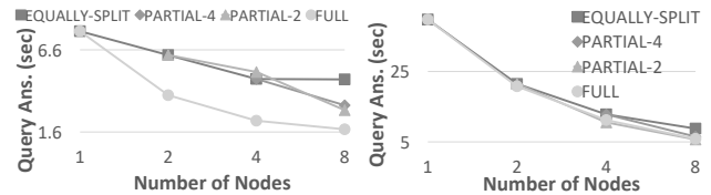
Figure 18: 10-NN query
