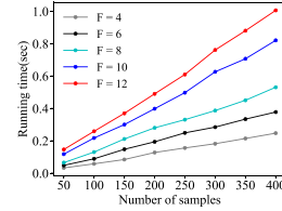
Figure 13: Running time of MagicScaler for scaling decisions vs. the number of samples.
