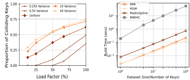
Figure 7: Effect of (1) gap distribution on LMH collisions (left), and (2) dataset size on building time (right).
