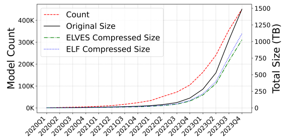
Figure 1: Increasing trend of model count (left Y) and aggregate storage size (right Y) of Hugging Face. “ELVES Compressed Size” or “ELF Compressed Size” represents the storage trend after ELVES alone or ELF alone is applied to Hugging Face’s PTM storage.
