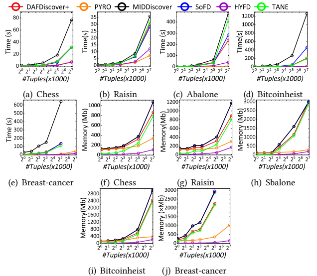
Figure 3: Scalability evaluation with varying data amounts
