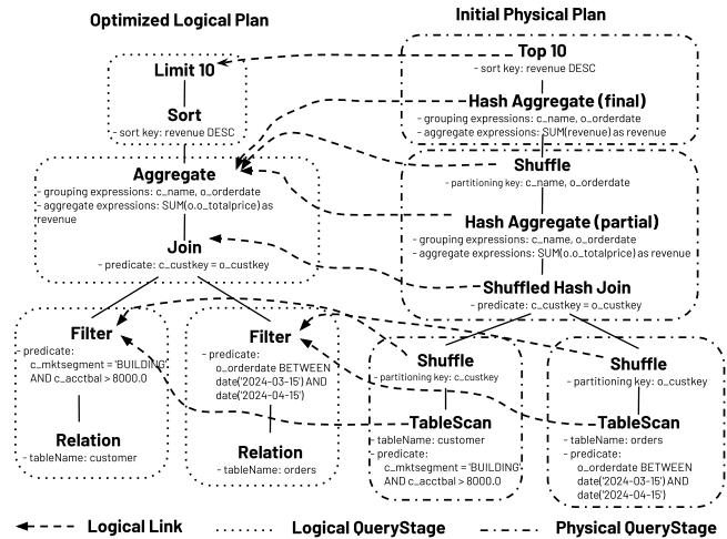
Figure 2: QueryStages and LogicalLinks
