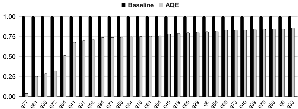
Figure 9: Performance Evaluations. "Baseline" is Photon with AQE-disabled, while "AQE" is Photon with AQE-enabled. For both Baseline and AQE, an experimental cluster has 1 i3.2xlarge driver with 16 i3.2xlarge executors. All queries run sequentially. All numbers are relative between Baseline and AQE. All numbers are the average from three replicated runs on dedicated clusters.
