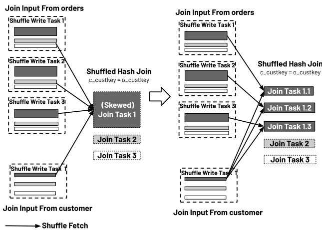
Figure 8: The Skew Join Rewrite Example
