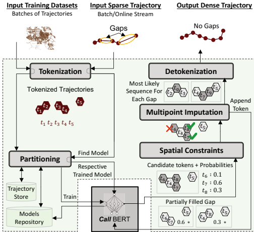
Figure 1: KAMEL Architecture
