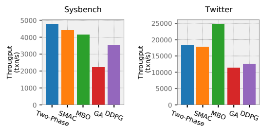
Figure 4: No Single Optimizer Dominates All Tuning Tasks – Performance of different optimizers on two workloads.
