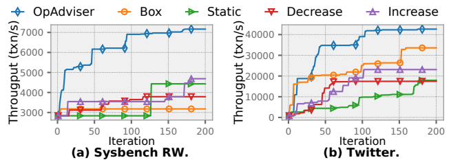
Figure 8: Comparison of Different Space Strategies.
