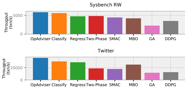
Figure 9: Comparison of Optimizer Selection Strategies.
