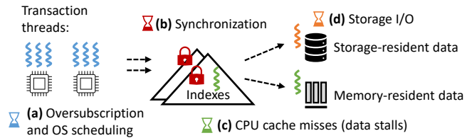
Figure 1: Main sources of latency in memory-optimized OLTP engines. Software prefetching can effectively hide data stalls (c). MosaicDB further mitigates the impact of other latencies (a, b, d) while preserving the benefits of software prefetching.
