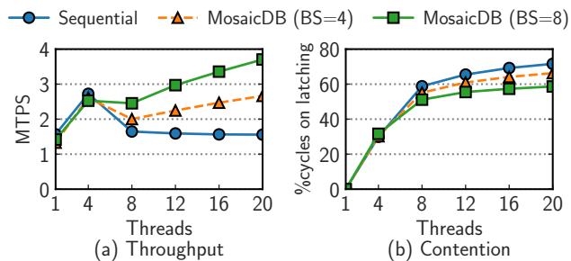
Figure 12: Throughput of a high-contention insert-only workload.
