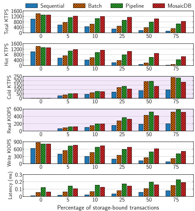
Figure 7: Read-write (50% read-only, 50% update-only) microbenchmark results under 10 threads and a varying percentage of storage-bound transactions.
