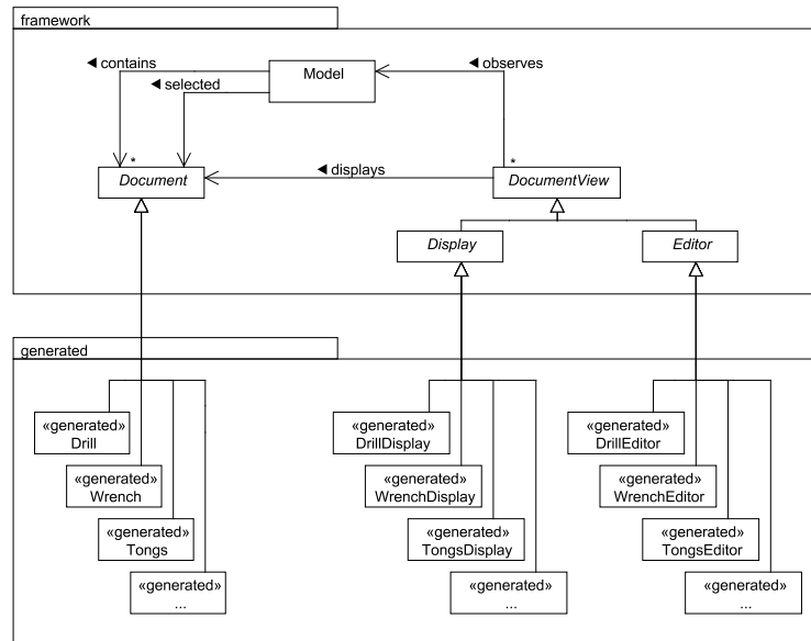
Fig. 5. Framework architecture
