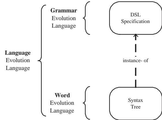
Figure 4. Evolution languages
