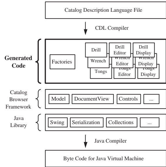
Figure 12. CDL stack
