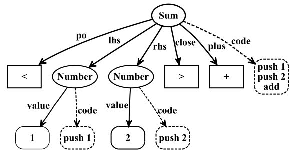
Figure 9. Syntax tree after transformation to postfix notation
