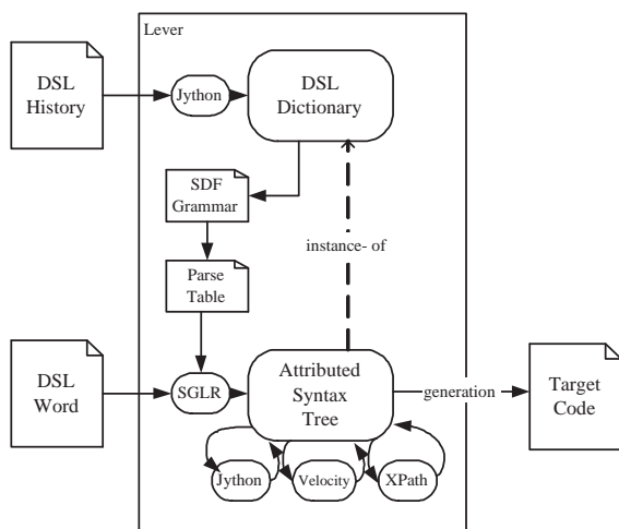
Figure 10. Lever implementation
