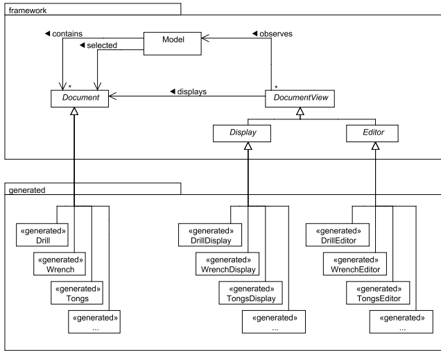
Figure 11. Framework architecture
