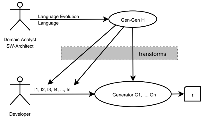
Figure 3. Generator-generator
