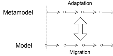
Fig. 1. Coupled evolution of metamodel and model
