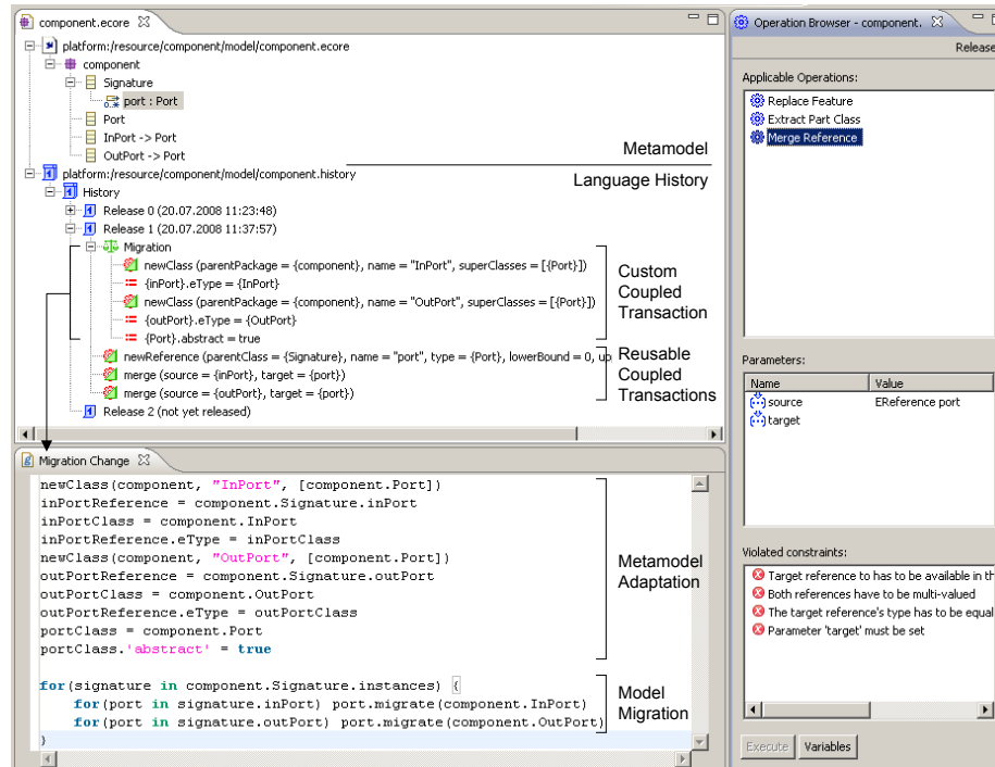
Fig. 5. Editor integration
