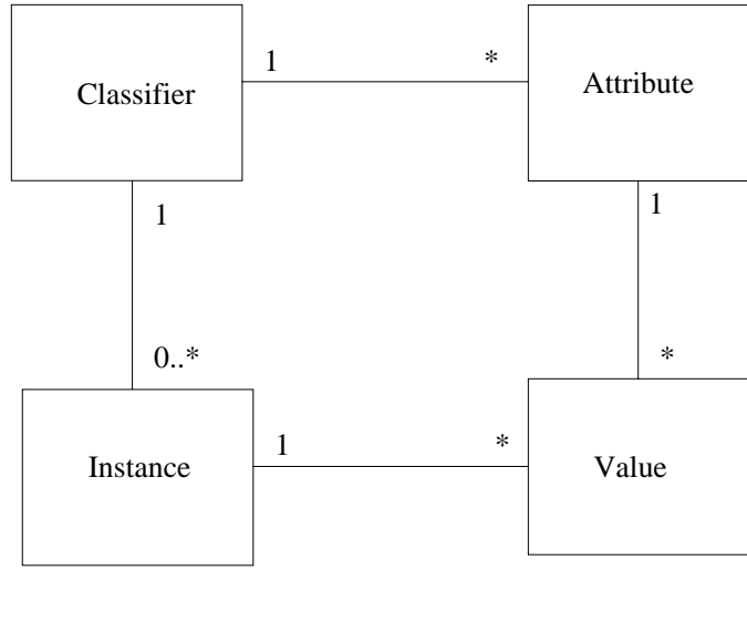
Figure 1: Class diagram representing syntax and partial semantics
