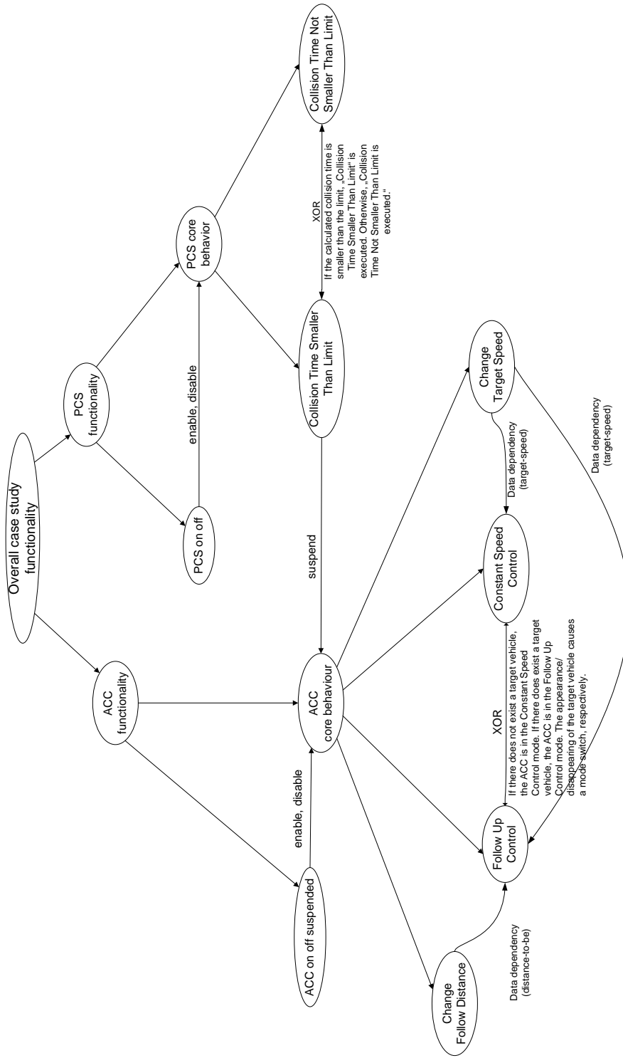
Figure 2: Service hierarchy
