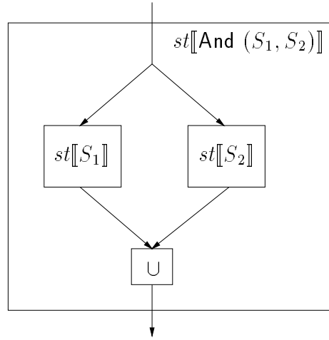
Figure 8: Parallel Composition
