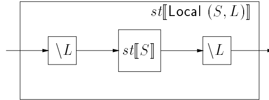
Figure 9: Local Signal-Scoping
