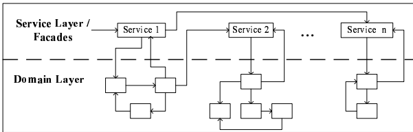
Figure 1: Service-Oriented Architectures
