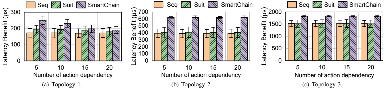
Figure 8. Latency benefit of SmartChain and two strawman solutions.
